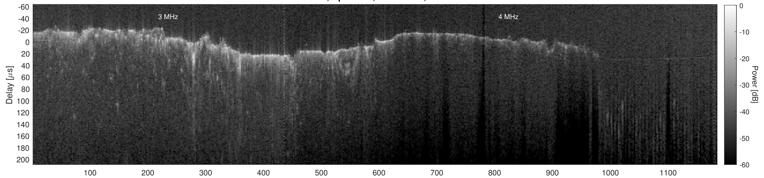
Orbit 10467, Cluttergram
