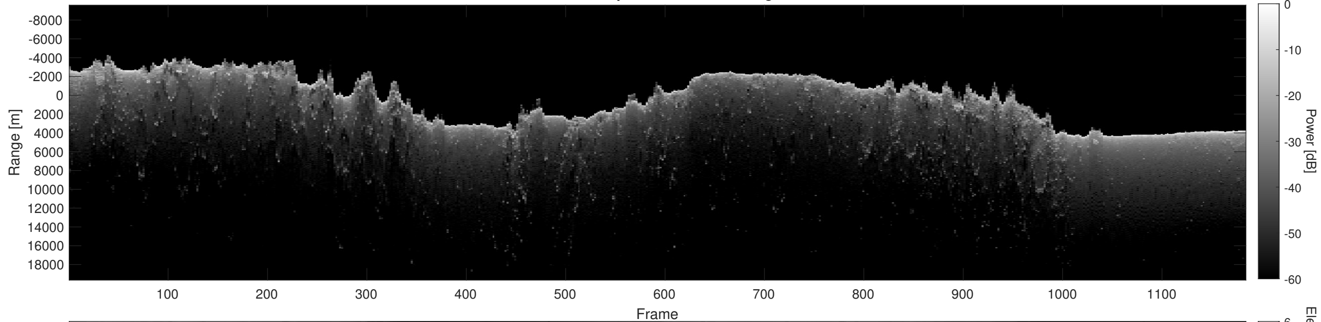
Orbit 10467, Depth-Corrected Cluttergram
