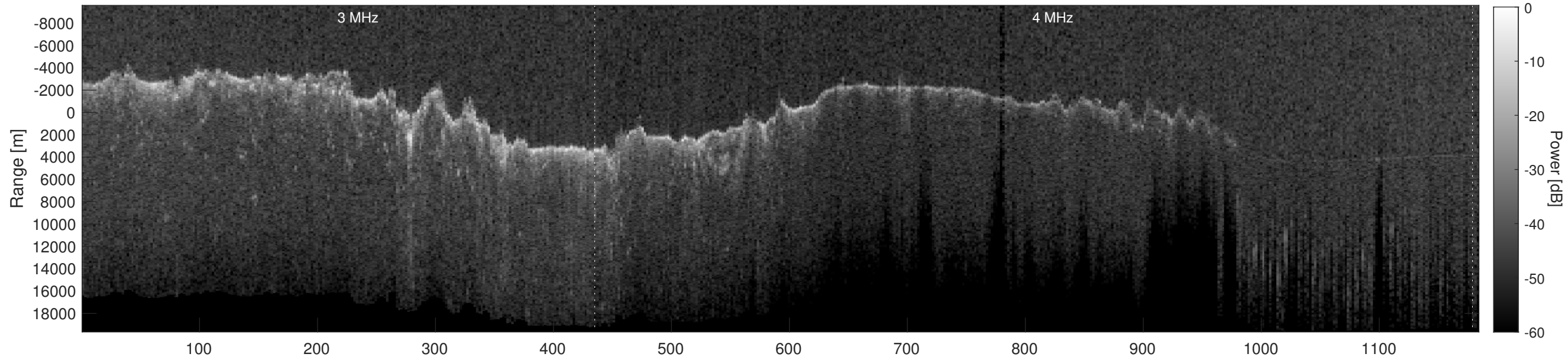
Orbit 10467, Depth-Corrected Cluttergram
