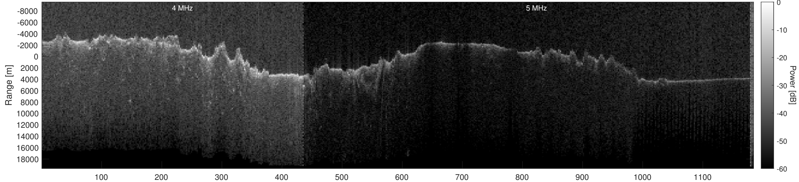
Orbit 10467, Optimized, Window, Depth-Corrected, Channel 2
