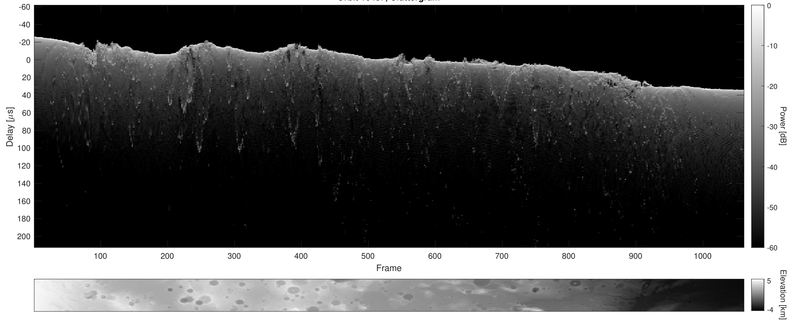
Orbit 10487, Cluttergram
