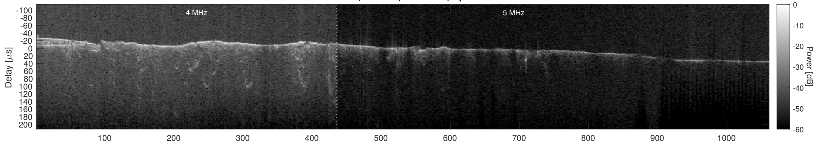
Orbit 10487, Cluttergram
