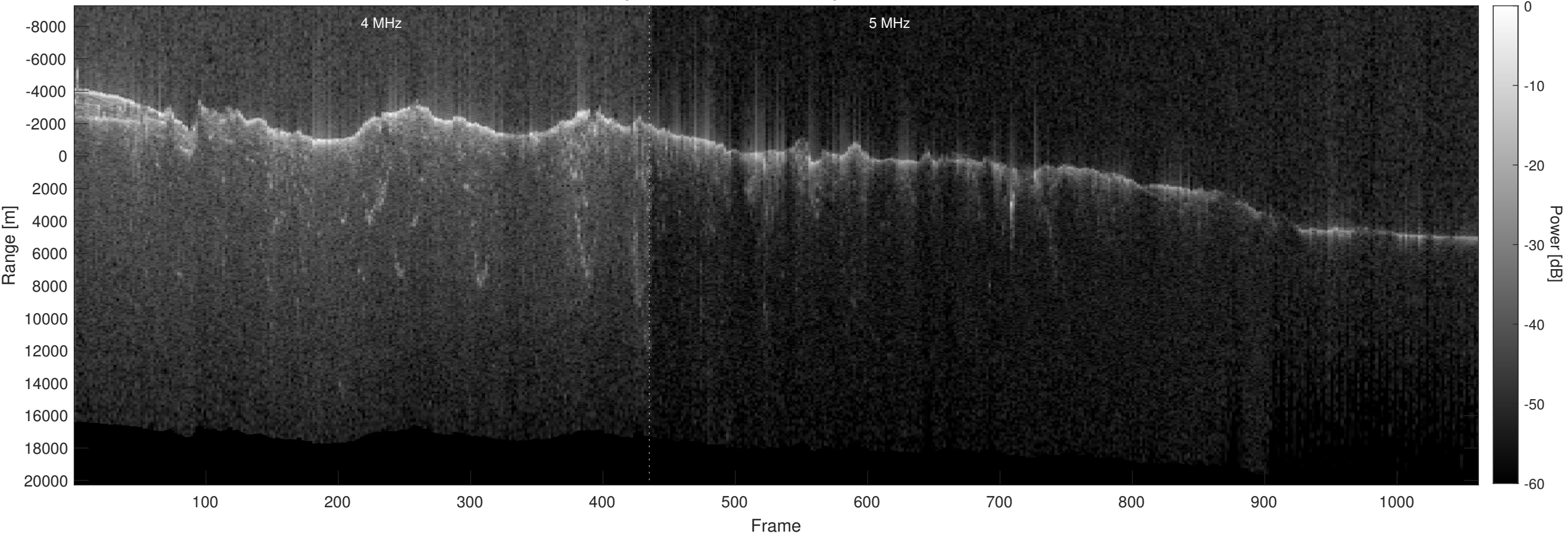
Orbit 10487, Optimized, No Window, Depth-Corrected, Channel 2
