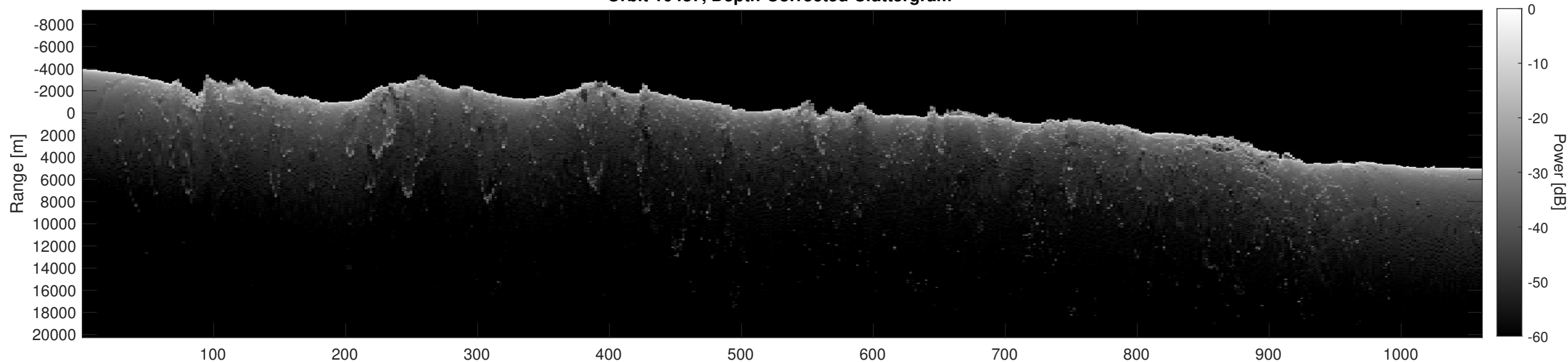
Orbit 10487, Depth-Corrected Cluttergram
