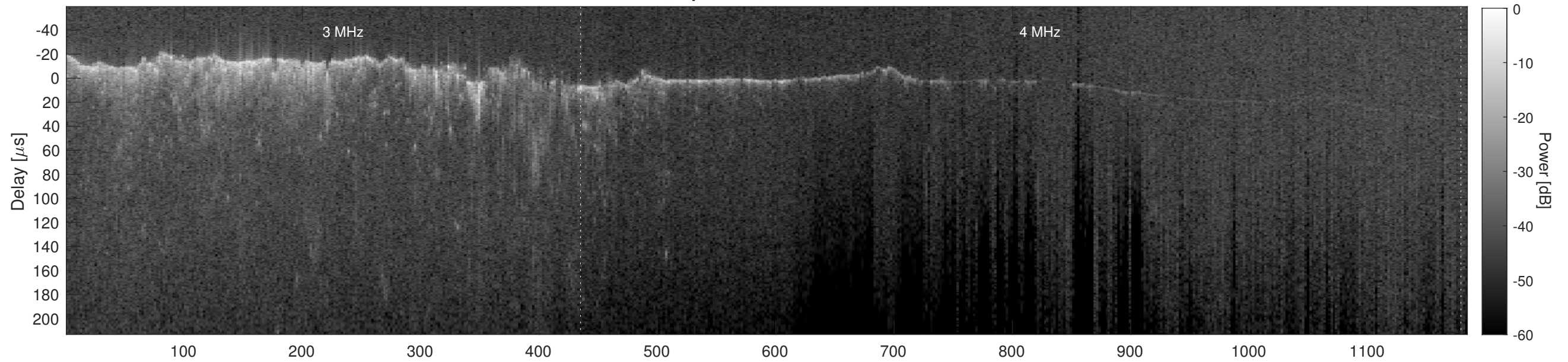
Orbit 10488, Cluttergram
