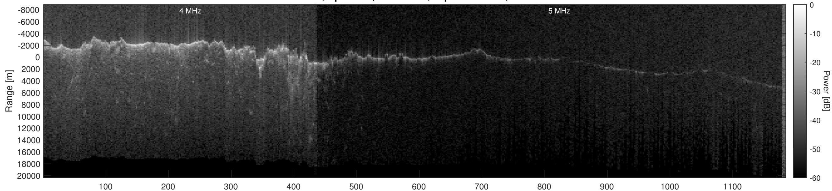
Orbit 10488, Optimized, No Window, Depth-Corrected, Channel 2
