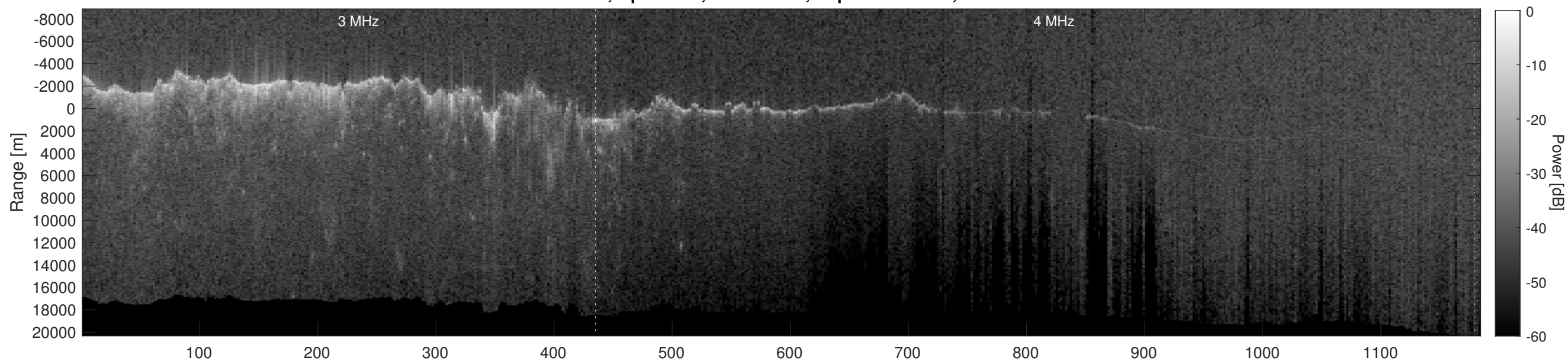
Orbit 10488, Depth-Corrected Cluttergram
