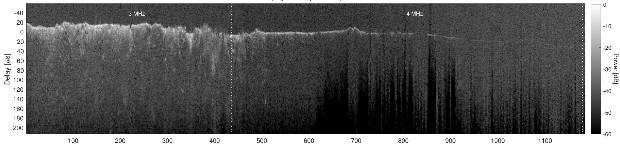
Orbit 10488, Cluttergram
