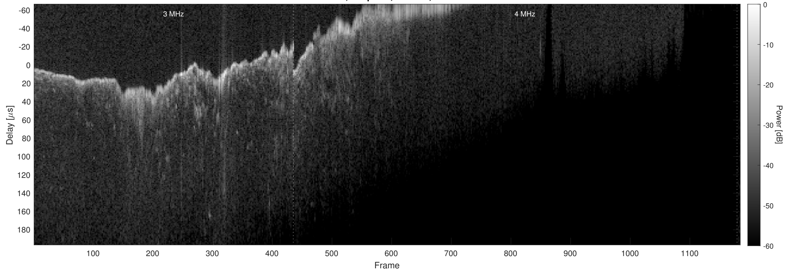
Orbit 10490, Chapman, Window, Channel 2
