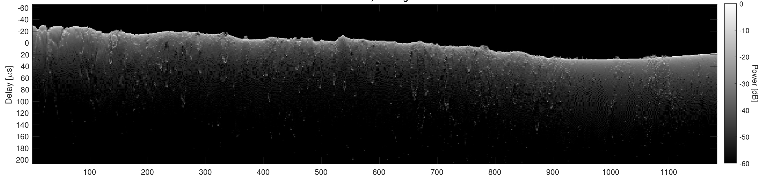
Orbit 10491, Cluttergram
