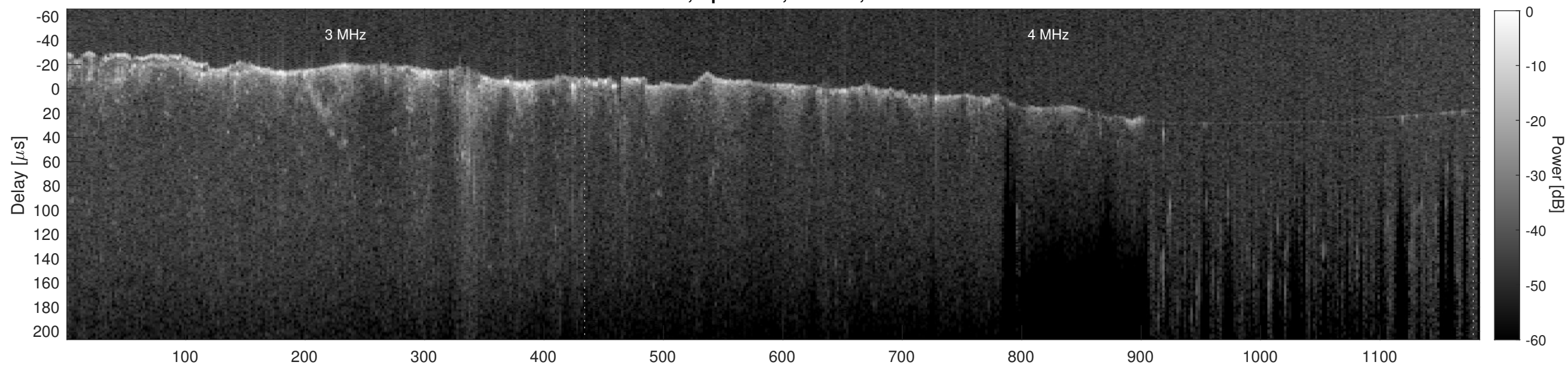
Orbit 10491, Cluttergram
