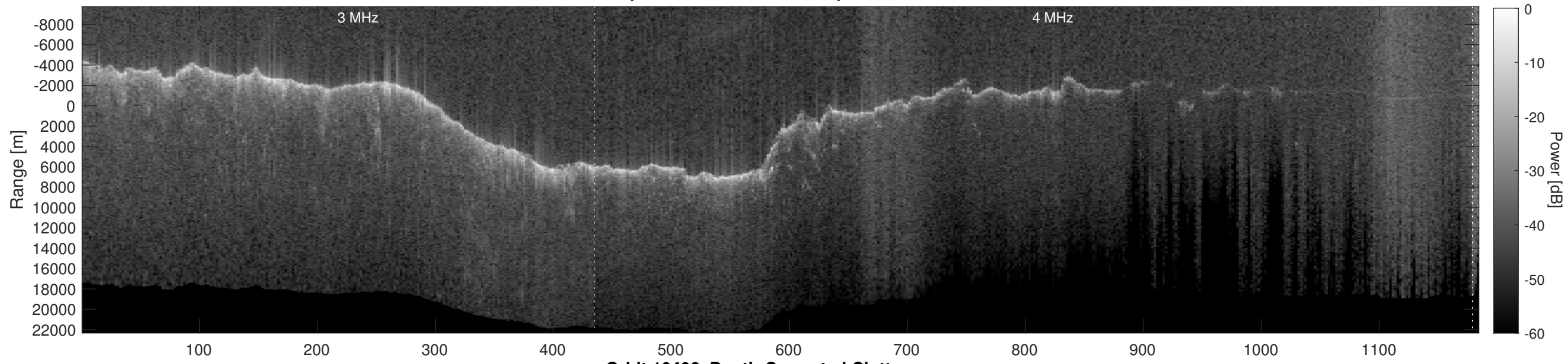
Orbit 10492, Depth-Corrected Cluttergram
