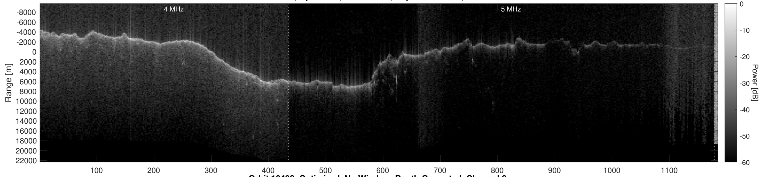
Orbit 10492, Optimized, No Window, Depth-Corrected, Channel 2
