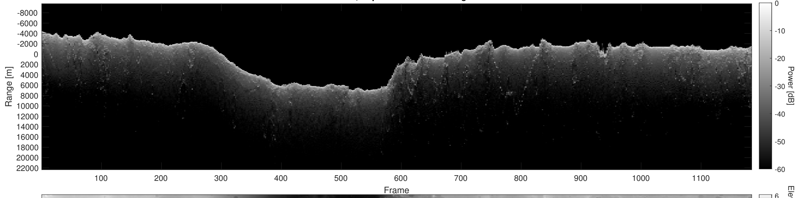
Orbit 10492, Depth-Corrected Cluttergram
