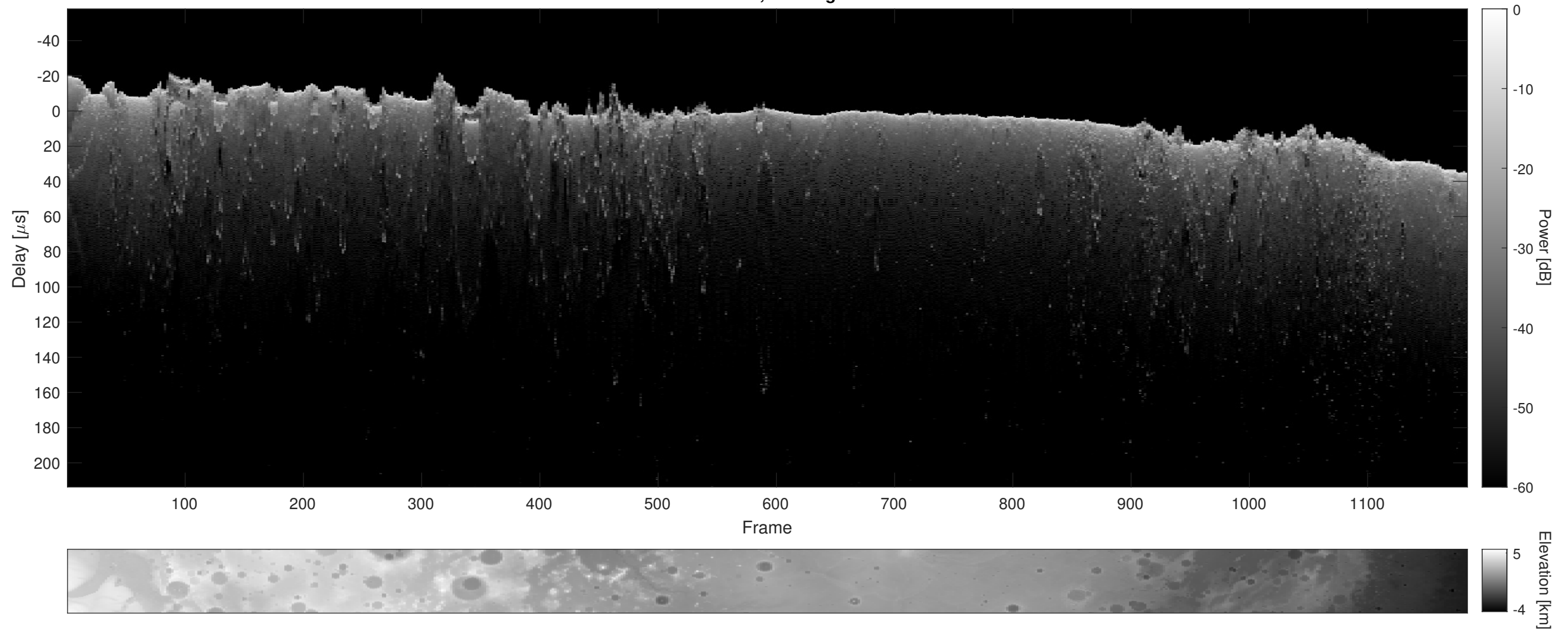
Orbit 10495, Cluttergram
