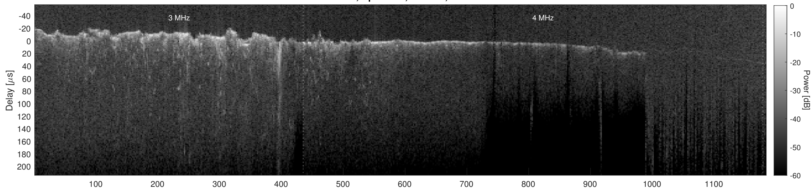
Orbit 10495, Cluttergram
