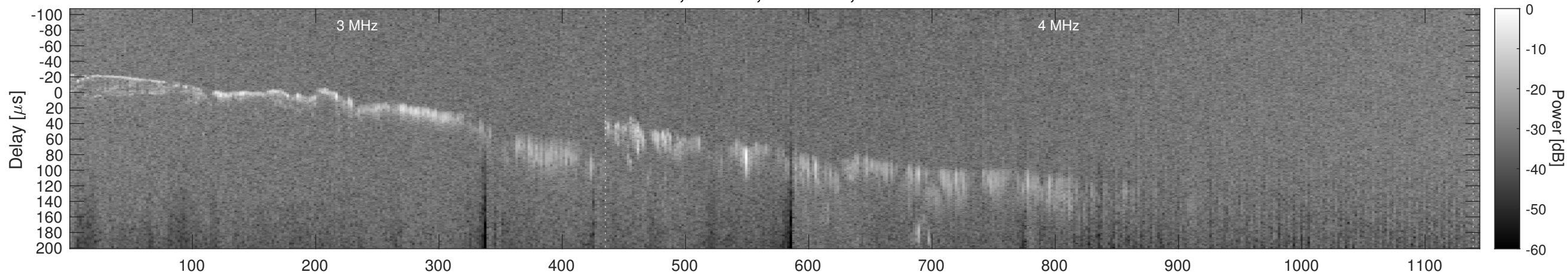
Orbit 10515, Window, Channel 2, Chapman
