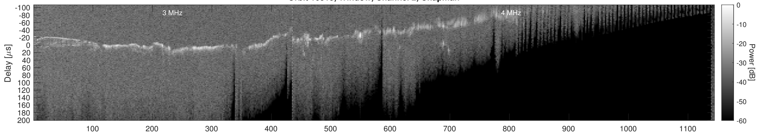
Orbit 10515, Window, Channel 2, Optimized
