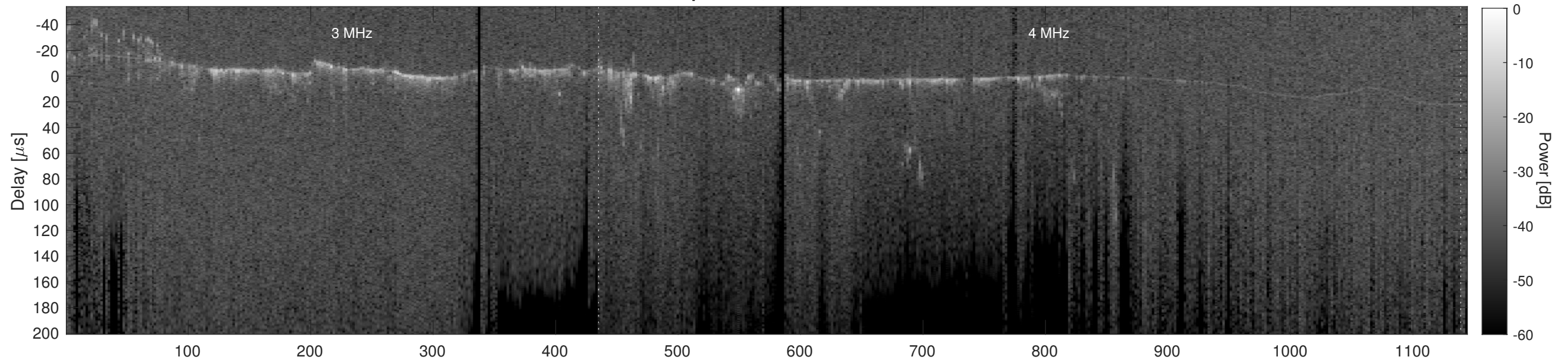
Orbit 10515, Cluttergram
