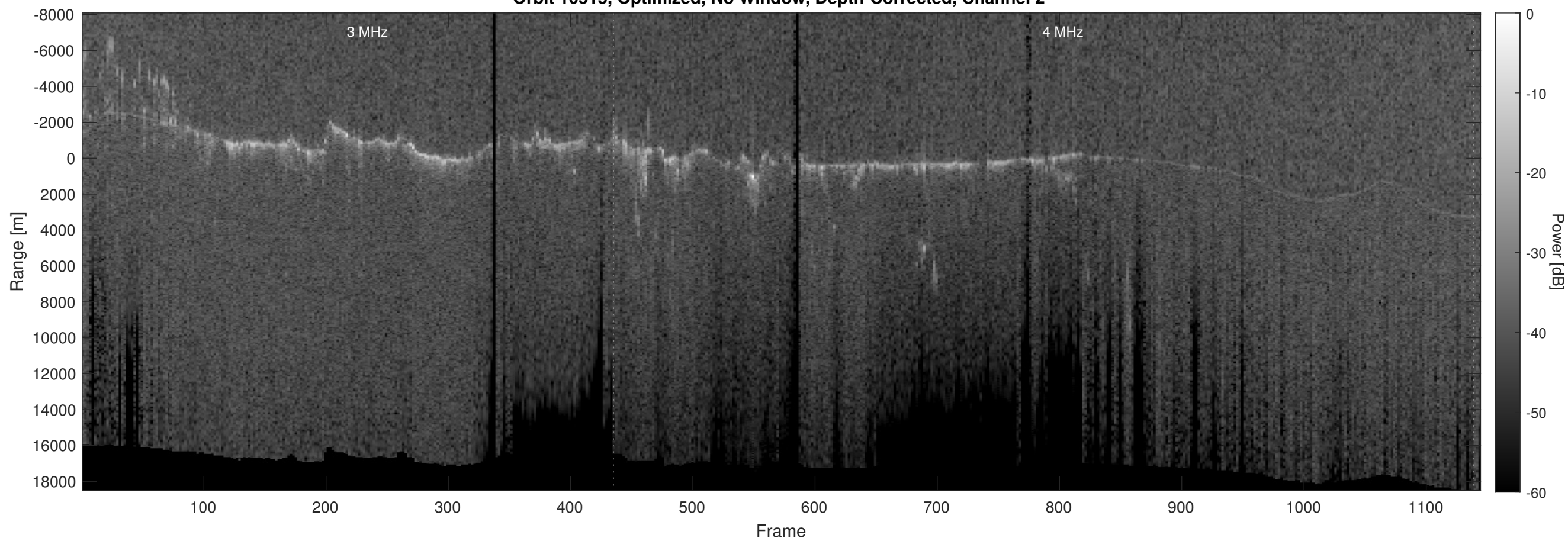
Orbit 10515, Optimized, No Window, Depth-Corrected, Channel 2
