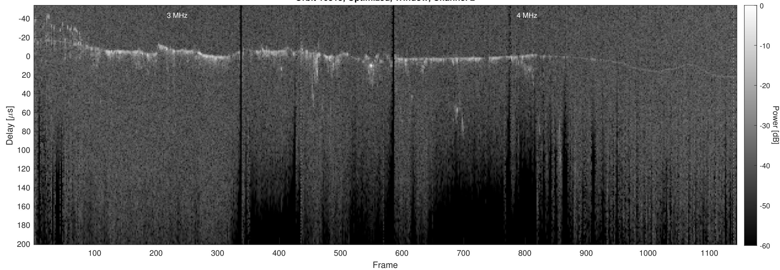
Orbit 10515, Optimized, Window, Channel 2
