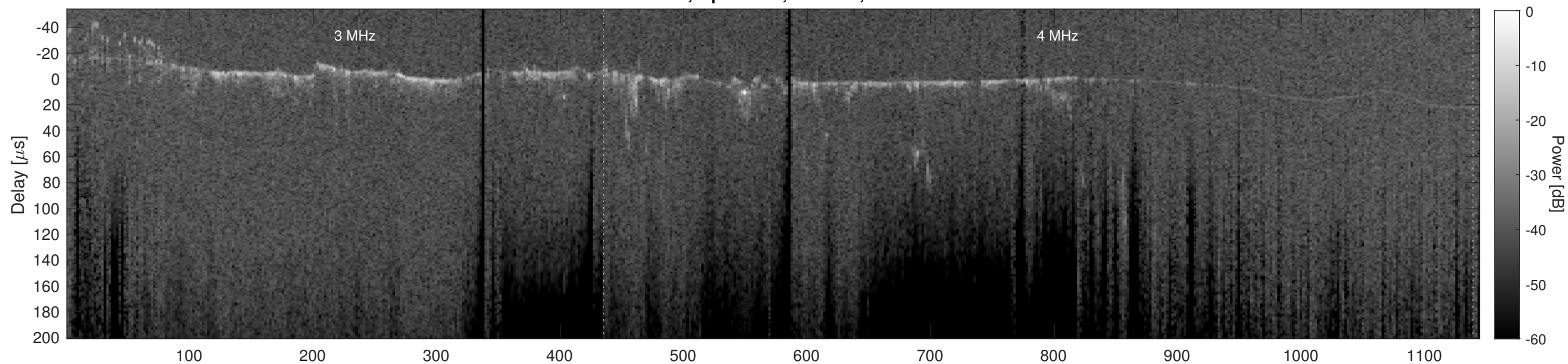
Orbit 10515, Cluttergram
