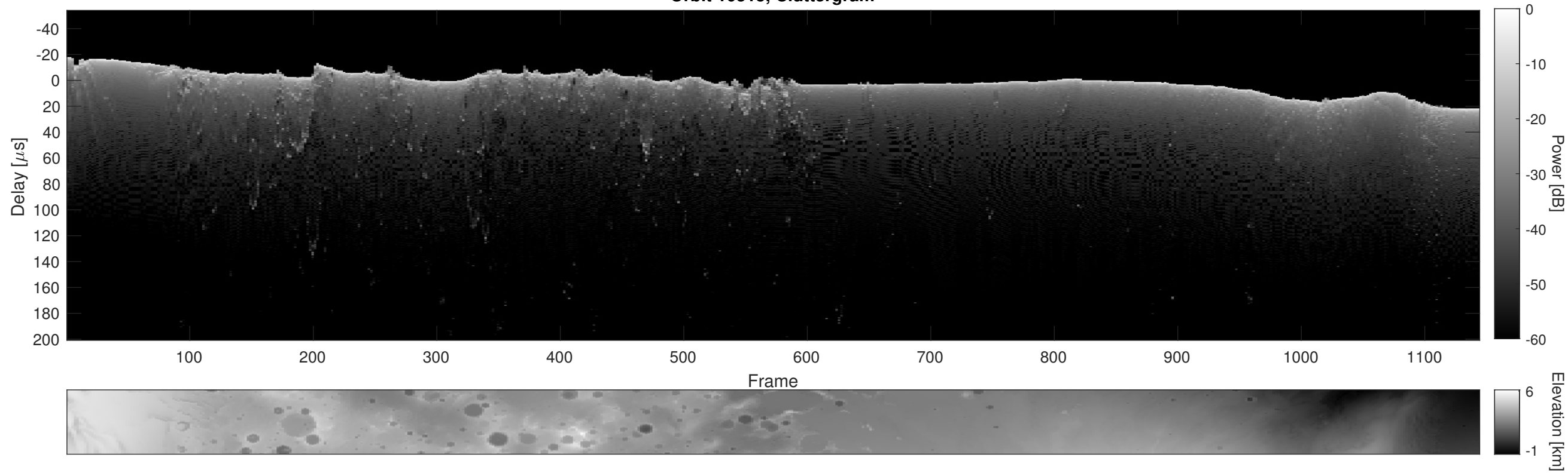
Orbit 10515, Cluttergram
