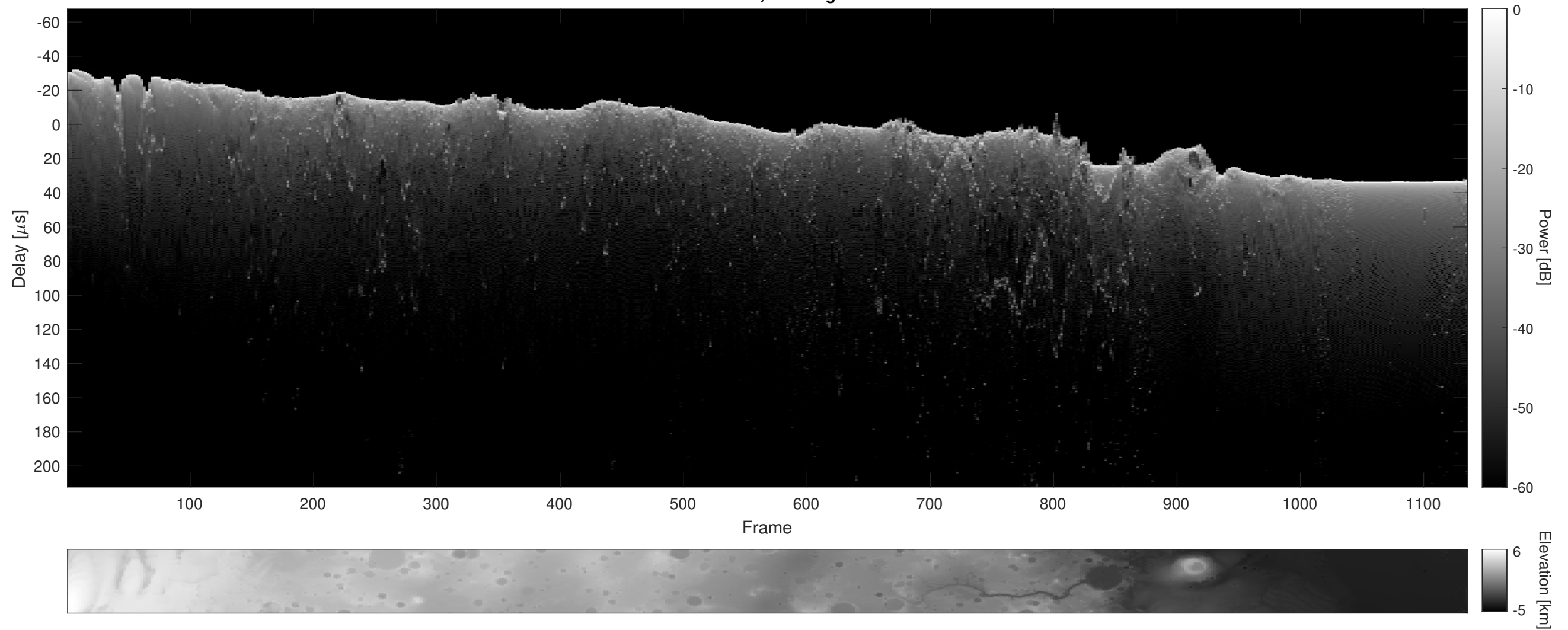
Orbit 10519, Cluttergram
