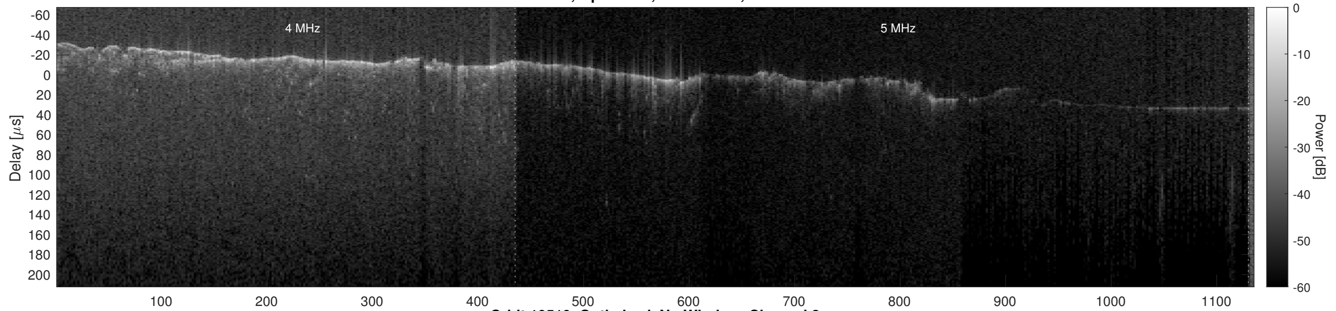
Orbit 10519, Optimized, No Window, Channel 2
