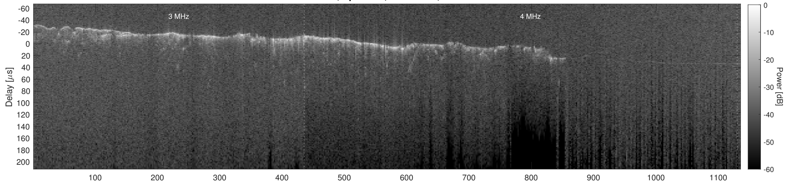
Orbit 10519, Cluttergram
