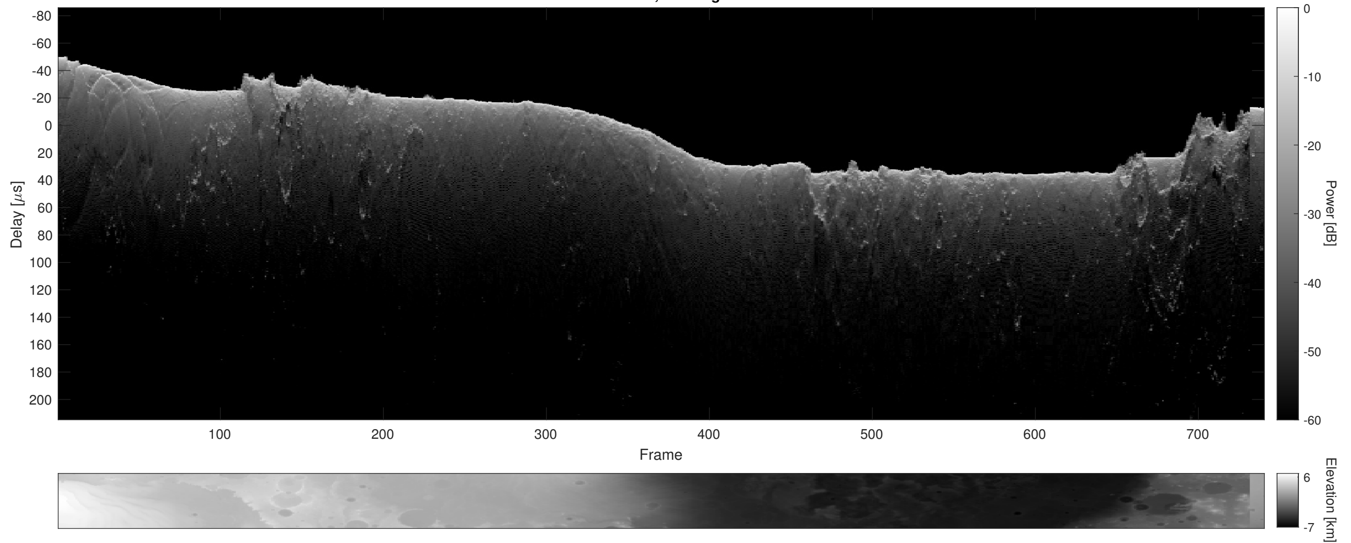
Orbit 10520, Cluttergram
