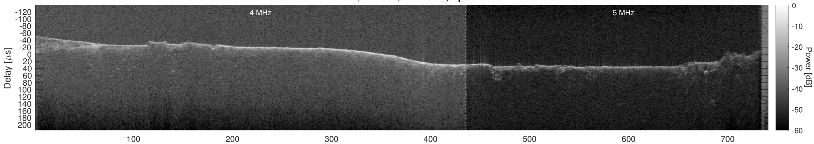
Orbit 10520, Cluttergram
