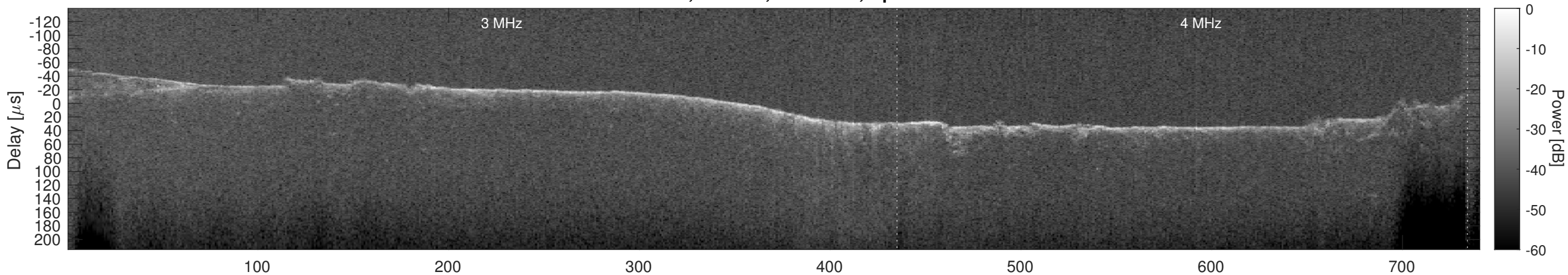
Orbit 10520, Cluttergram
