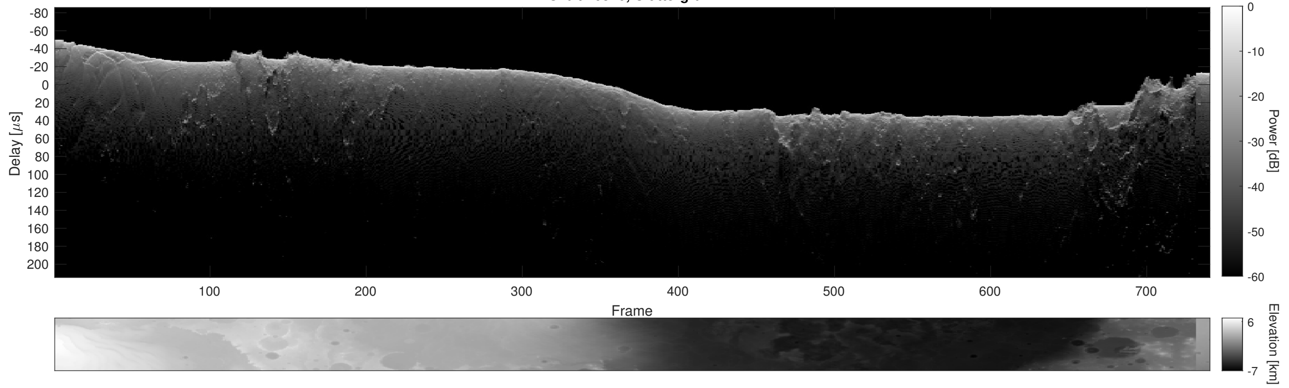
Orbit 10520, Cluttergram
