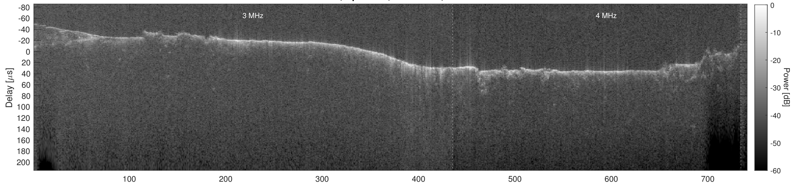
Orbit 10520, Cluttergram
