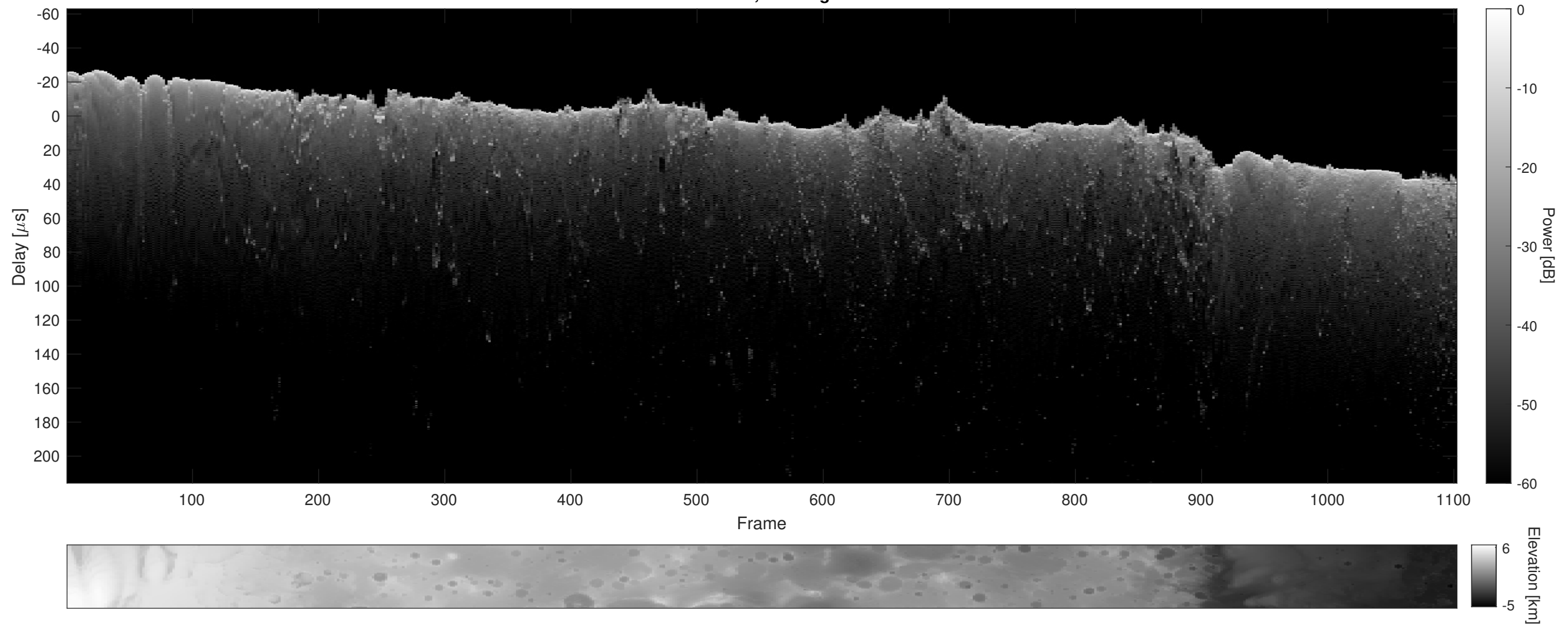
Orbit 10533, Cluttergram
