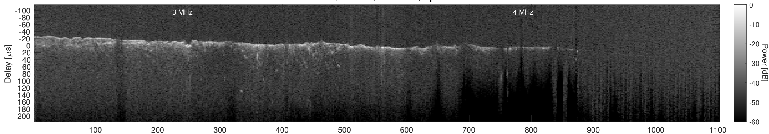
Orbit 10533, Cluttergram
