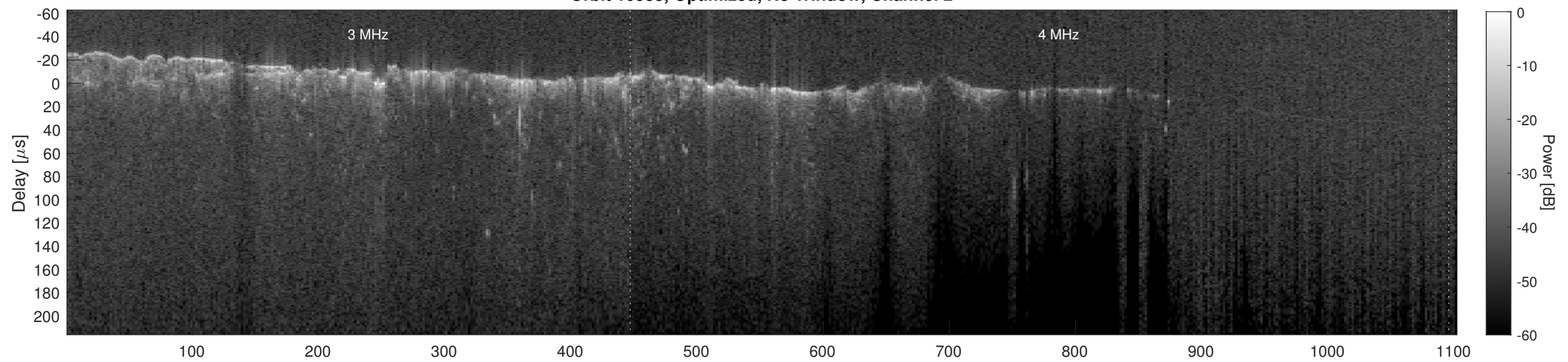
Orbit 10533, Cluttergram
