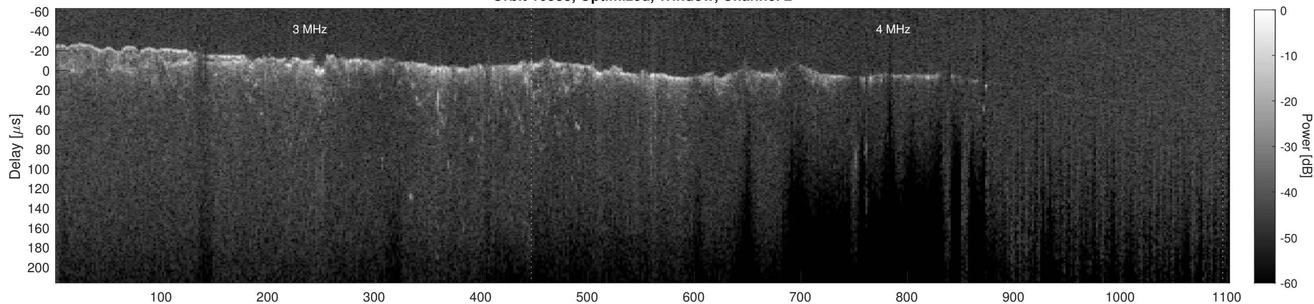
Orbit 10533, Cluttergram
