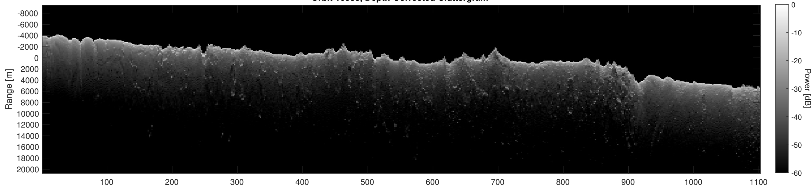
Orbit 10533, Depth-Corrected Cluttergram
