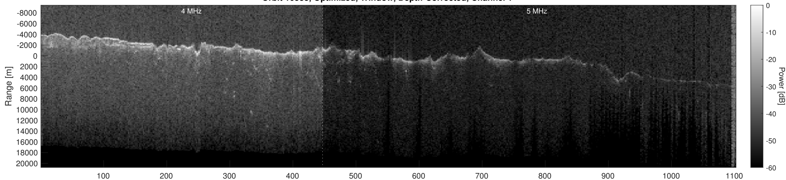
Orbit 10533, Optimized, Window, Depth-Corrected, Channel 2
