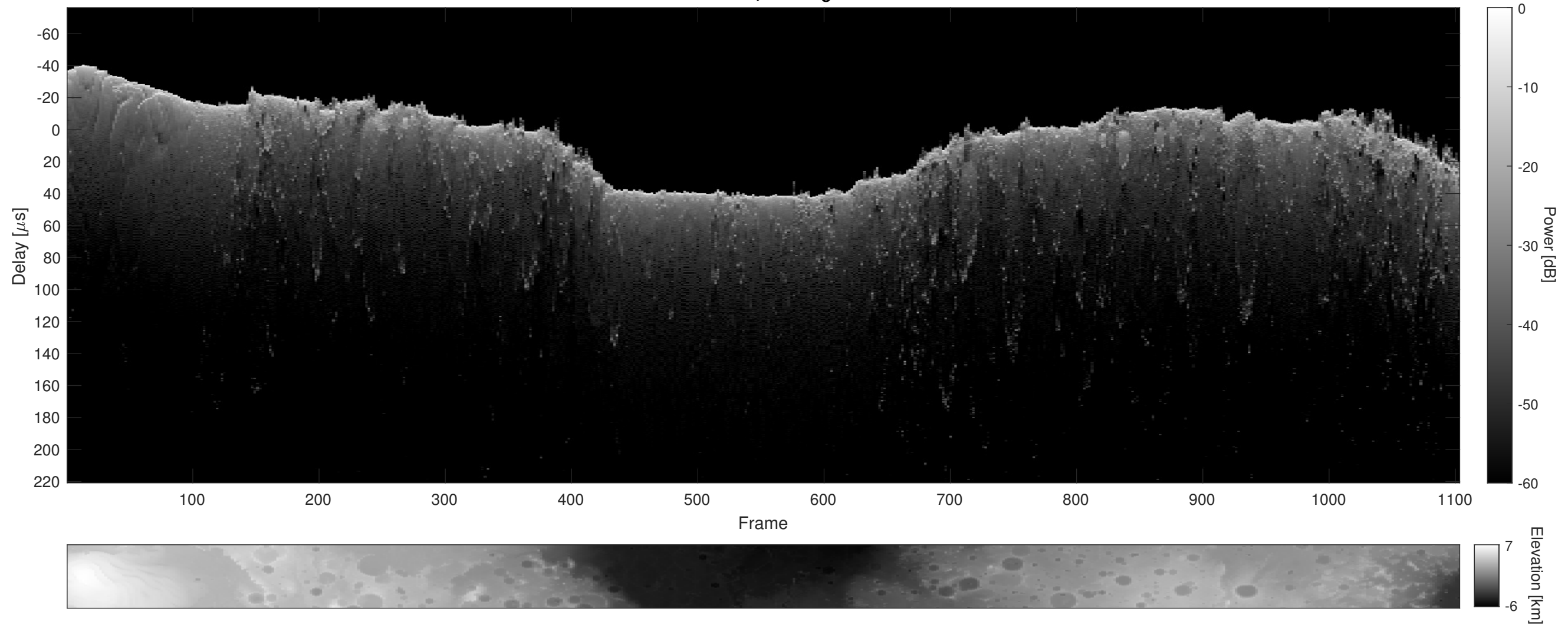
Orbit 10534, Cluttergram
