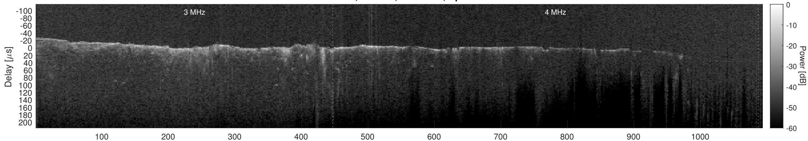
Orbit 10537, Cluttergram
