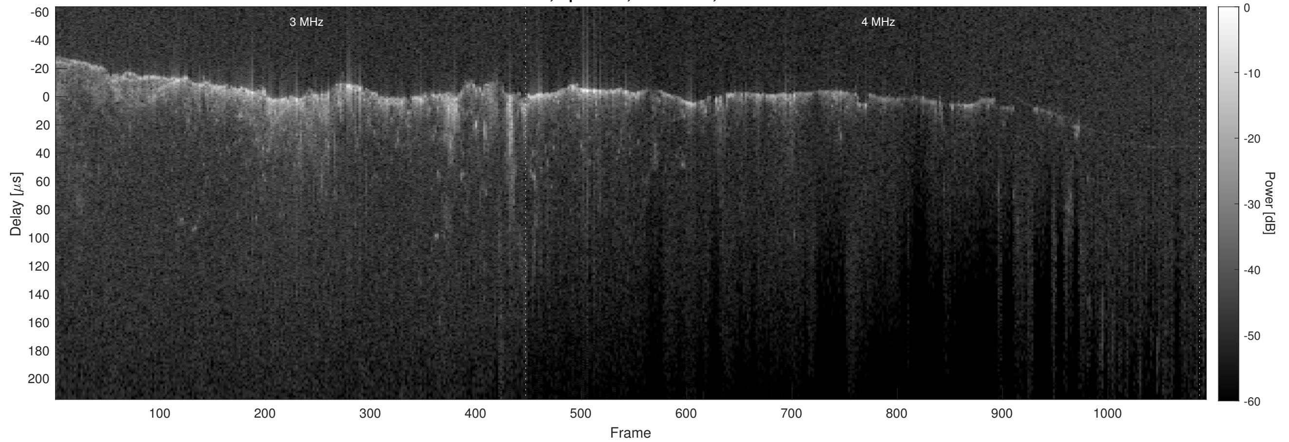
Orbit 10537, Optimized, No Window, Channel 2
