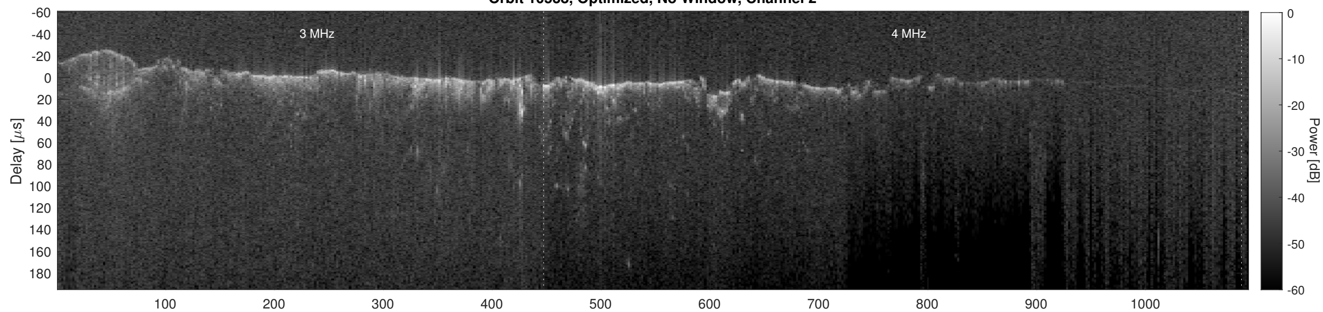
Orbit 10538, Cluttergram
