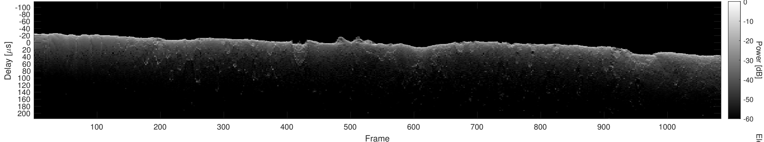
Orbit 10540, Cluttergram
