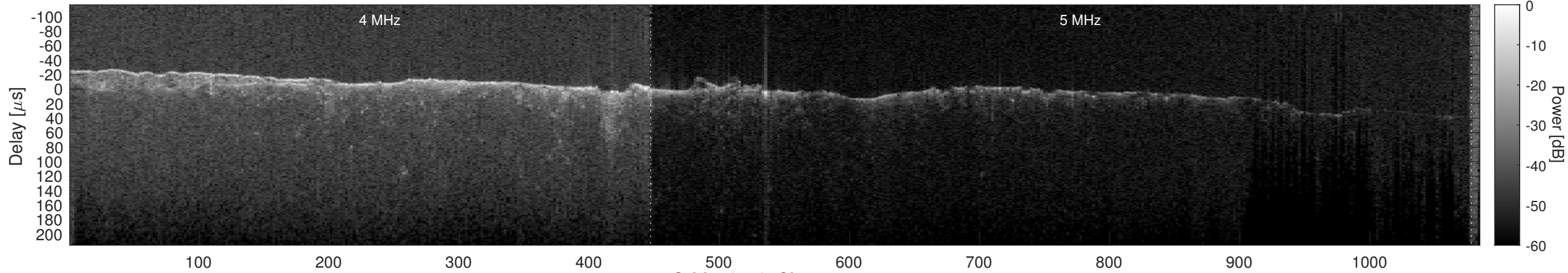
Orbit 10540, Cluttergram
