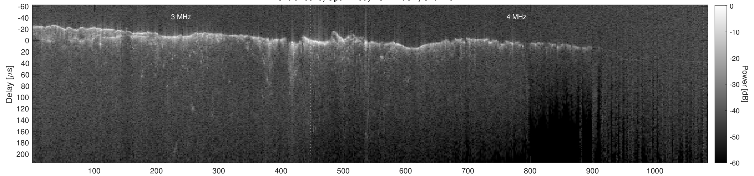
Orbit 10540, Cluttergram
