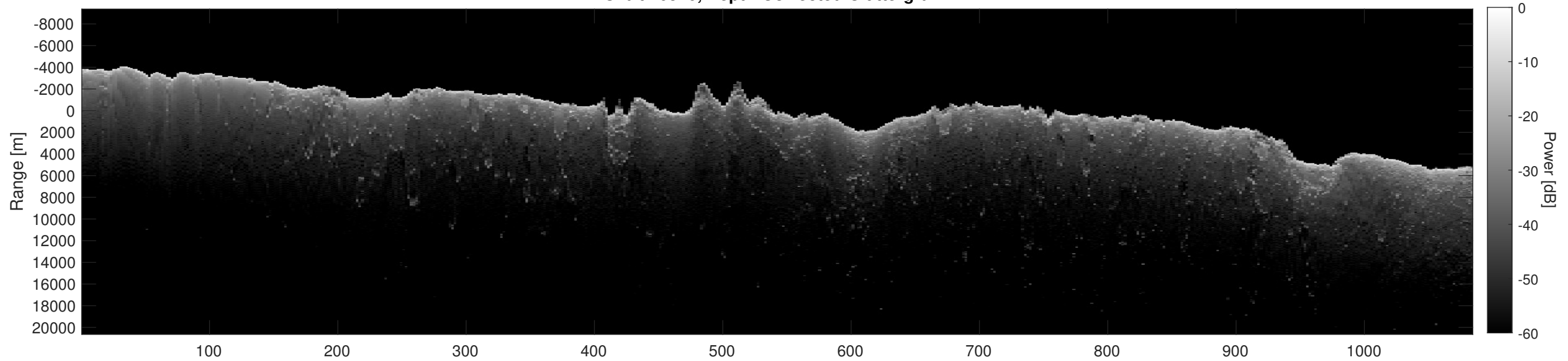
Orbit 10540, Depth-Corrected Cluttergram
