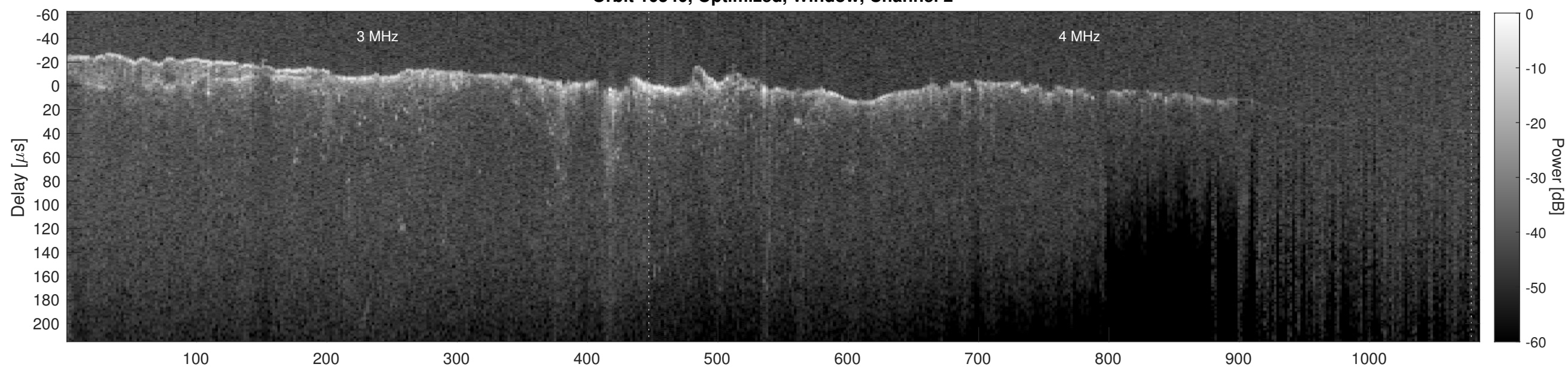
Orbit 10540, Cluttergram
