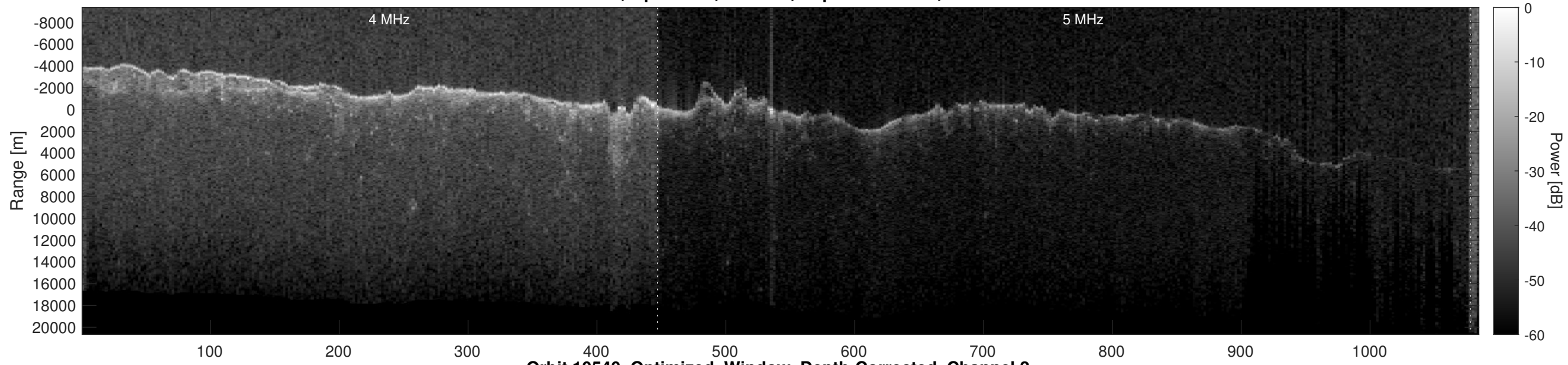
Orbit 10540, Optimized, Window, Depth-Corrected, Channel 2
