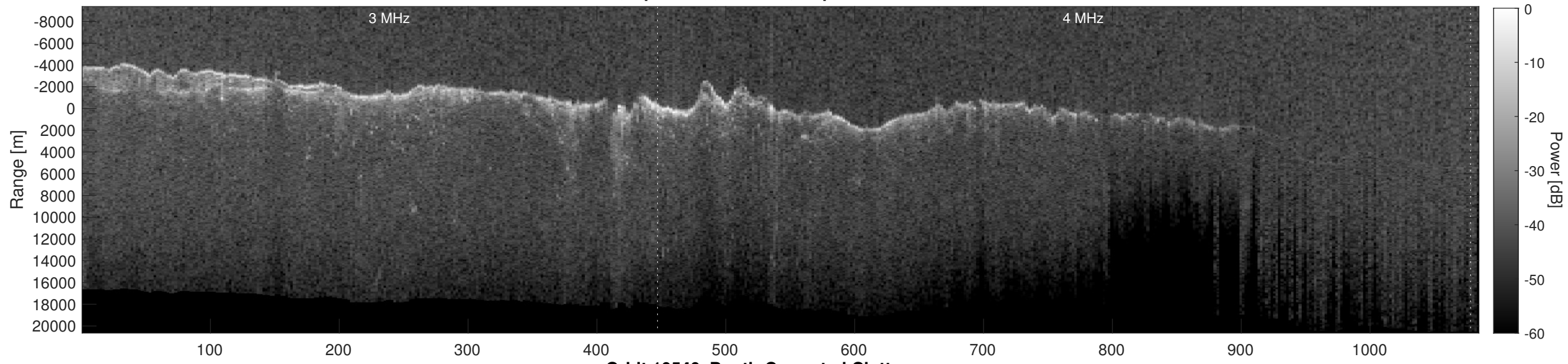
Orbit 10540, Depth-Corrected Cluttergram
