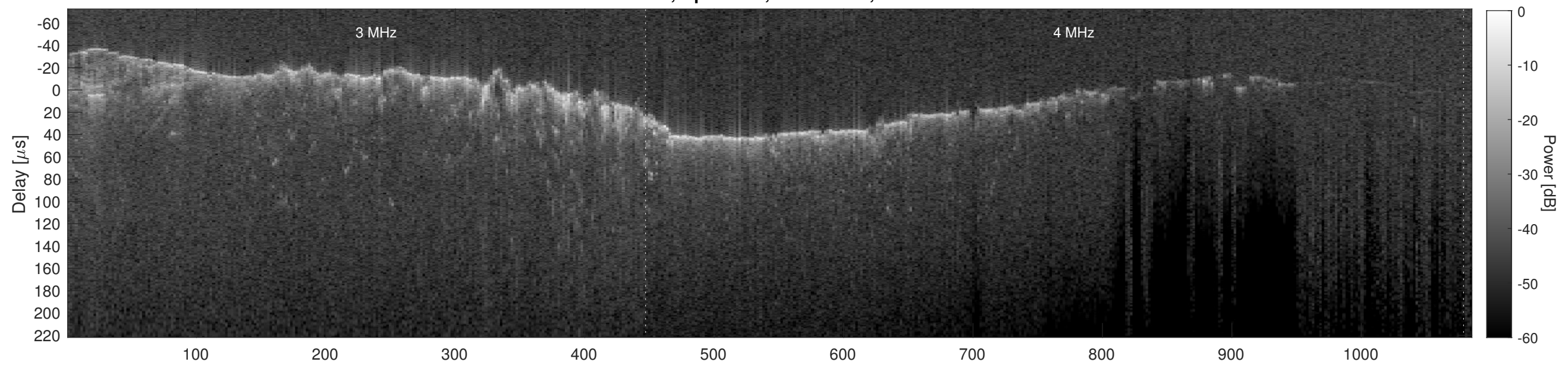
Orbit 10541, Cluttergram
