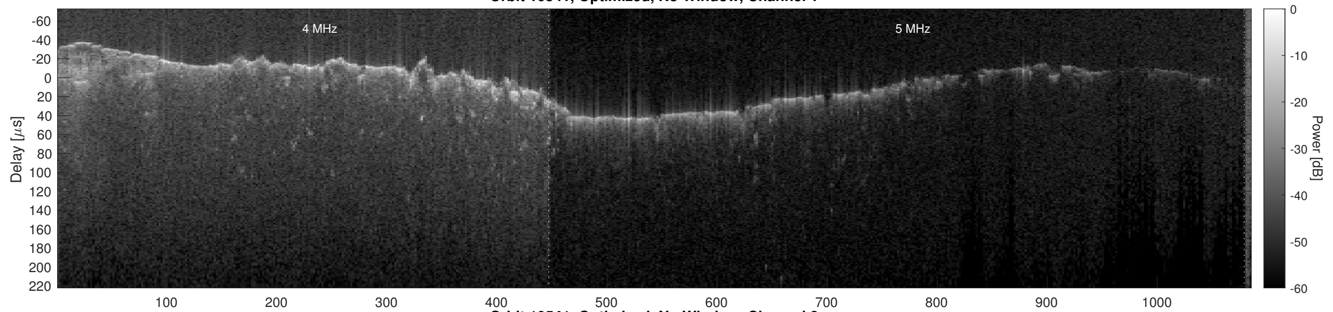
Orbit 10541, Optimized, No Window, Channel 2
