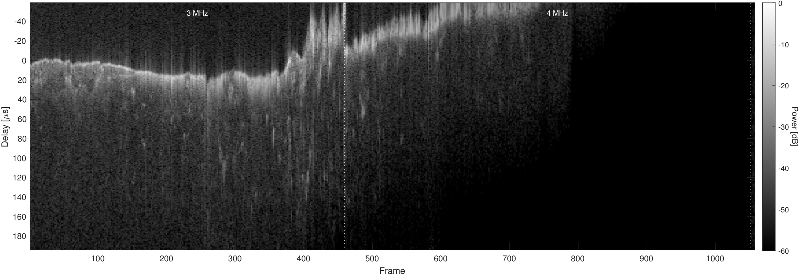
Orbit 10557, Chapman, No Window, Channel 2
