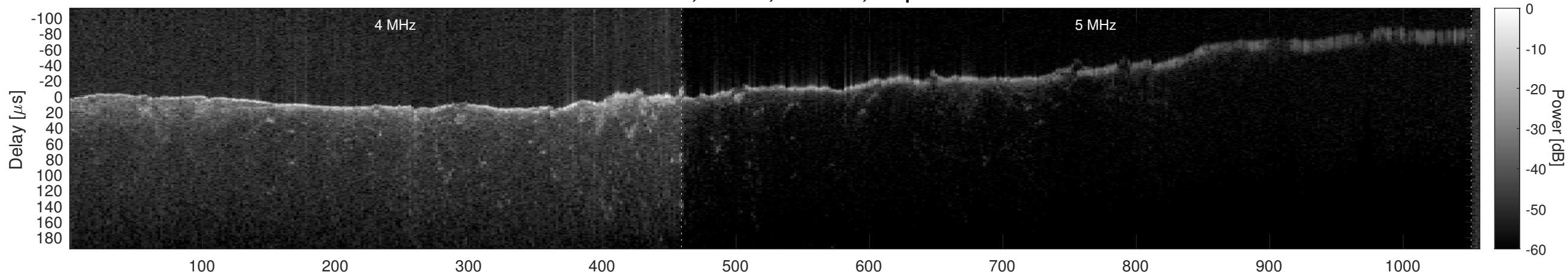
Orbit 10557, Window, Channel 1, Optimized
