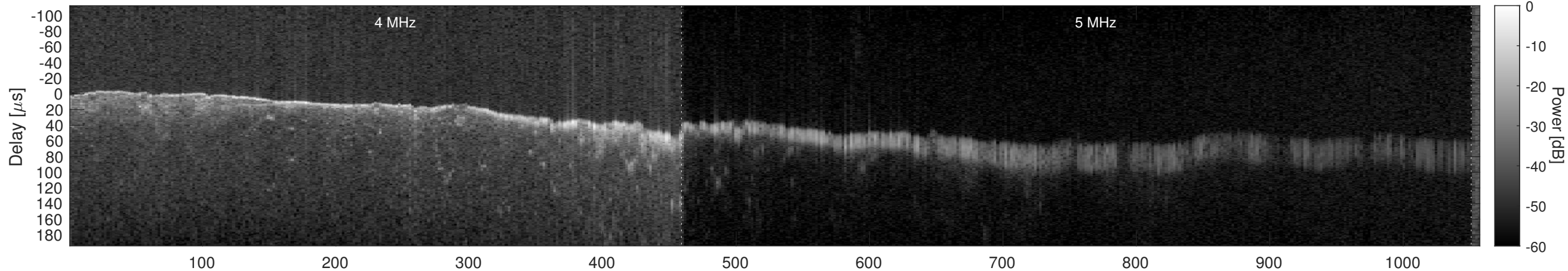
Orbit 10557, Window, Channel 1, Chapman
