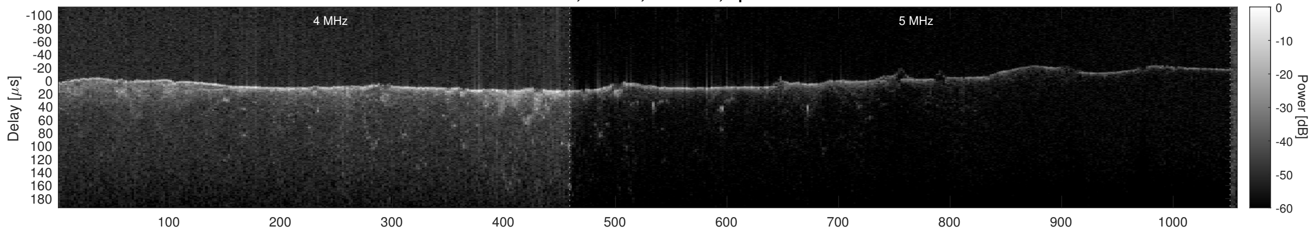
Orbit 10557, Cluttergram
