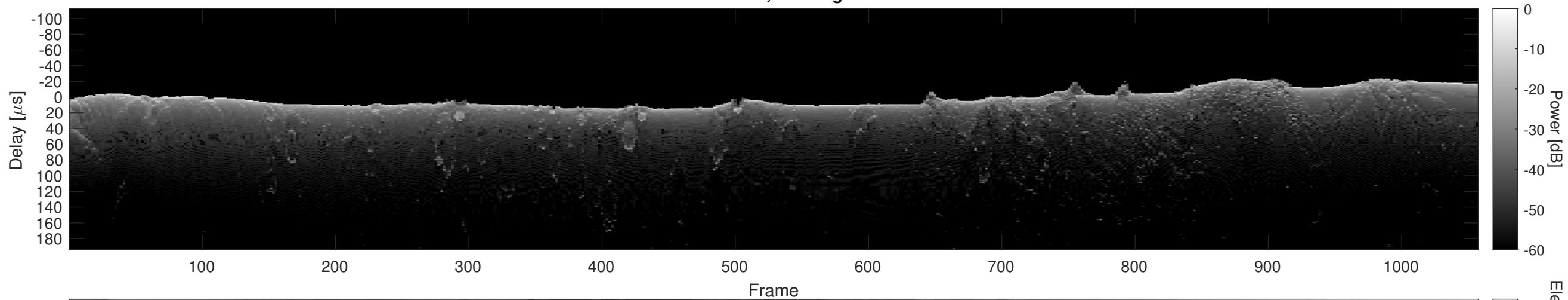
Orbit 10557, Cluttergram
