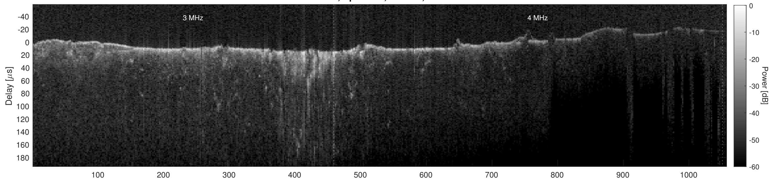
Orbit 10557, Cluttergram
