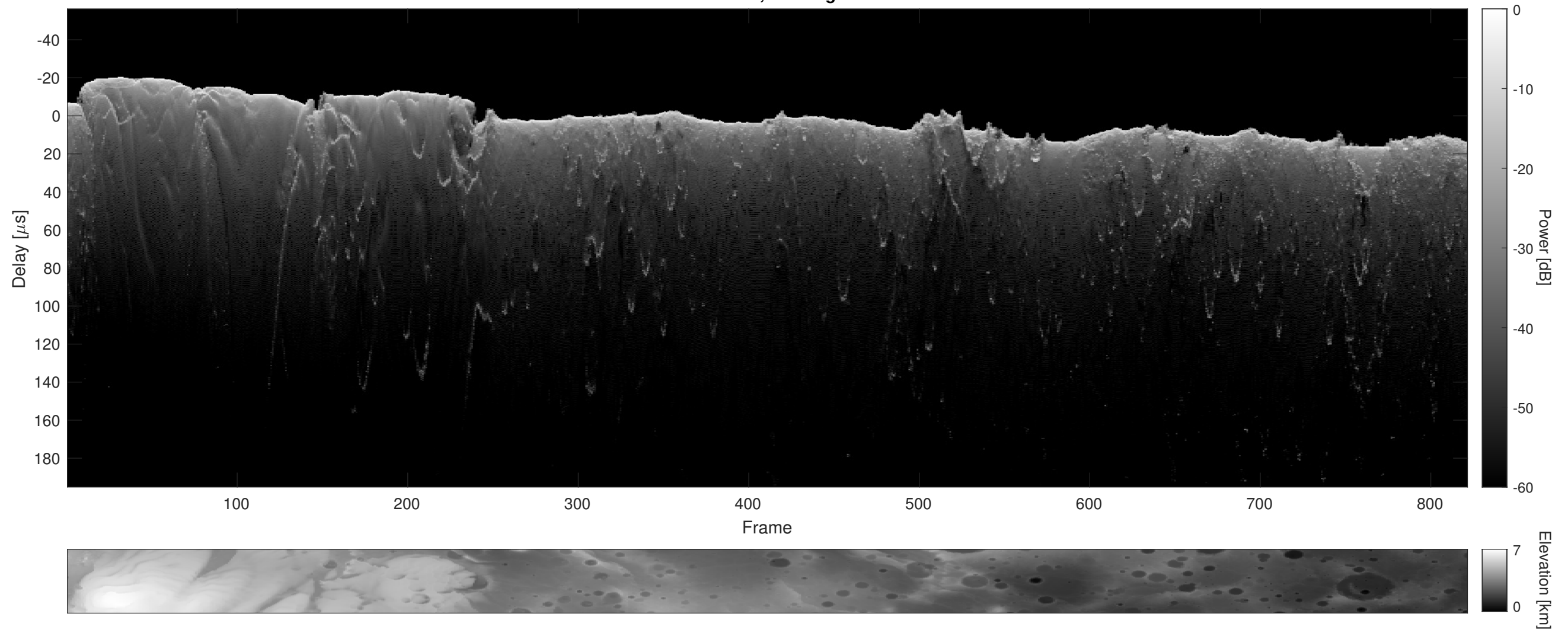
Orbit 10558, Cluttergram
