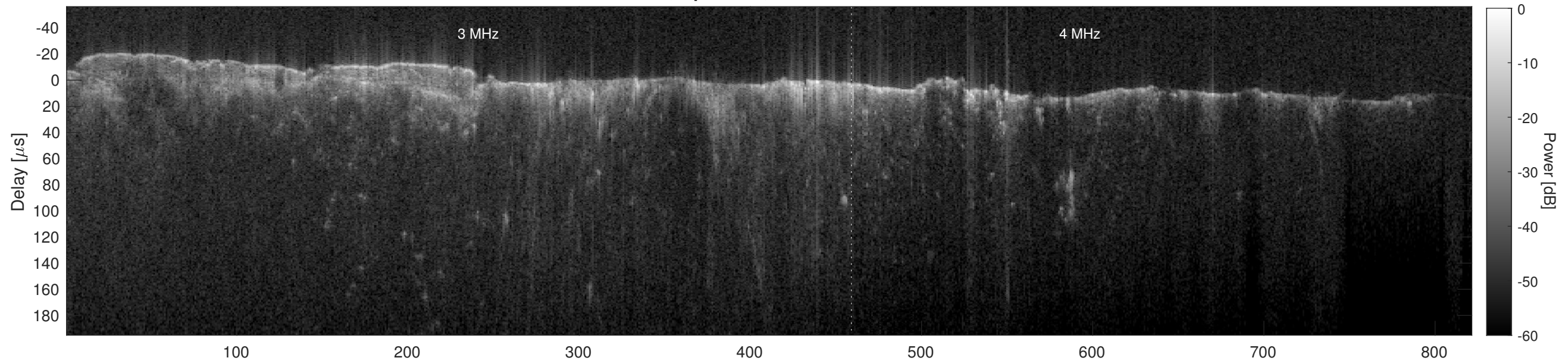
Orbit 10558, Cluttergram
