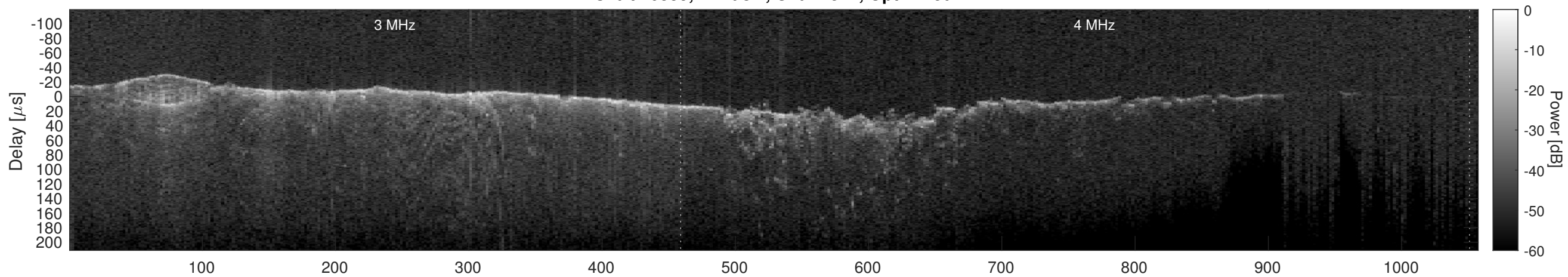
Orbit 10559, Cluttergram
