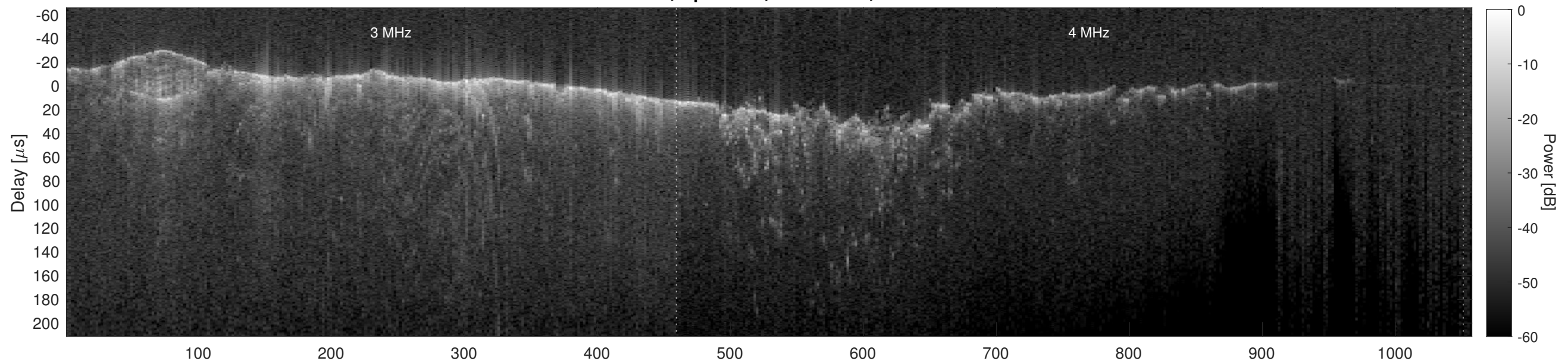
Orbit 10559, Cluttergram
