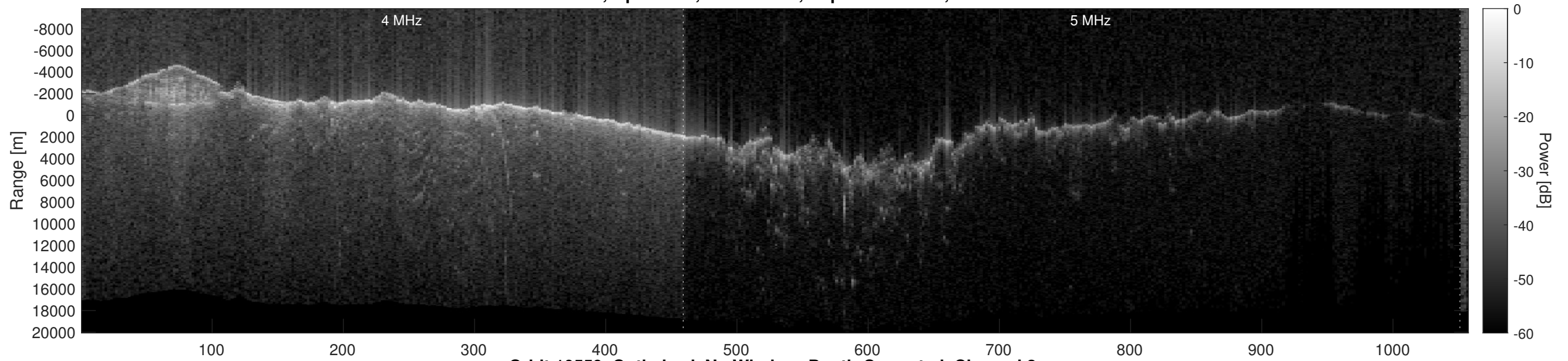
Orbit 10559, Optimized, No Window, Depth-Corrected, Channel 2
